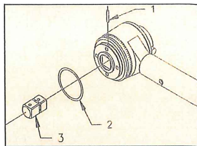
Figure 1. Replacing Output Square Drive Assembly
